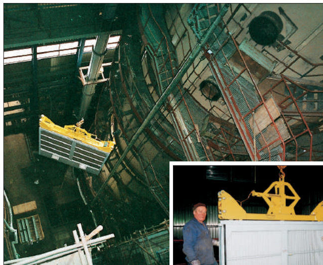
LTH 100 beeing installed in a flue-gas desulphurization plant
