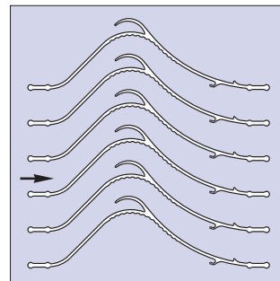
LTH 100 profile geometry
