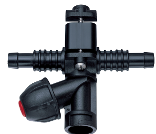
Hose connection double For pipe outside dia. 3/4" (25–28 mm O.D.) 065.275.56.KL For pipe outside dia. 1/2" (20–22 mm O.D.) 065.275.56.KH
