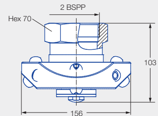
Female thread
