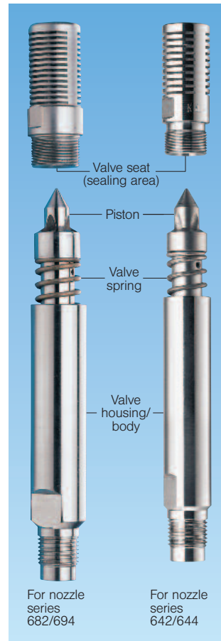
WSV Water Stop Valve, components
