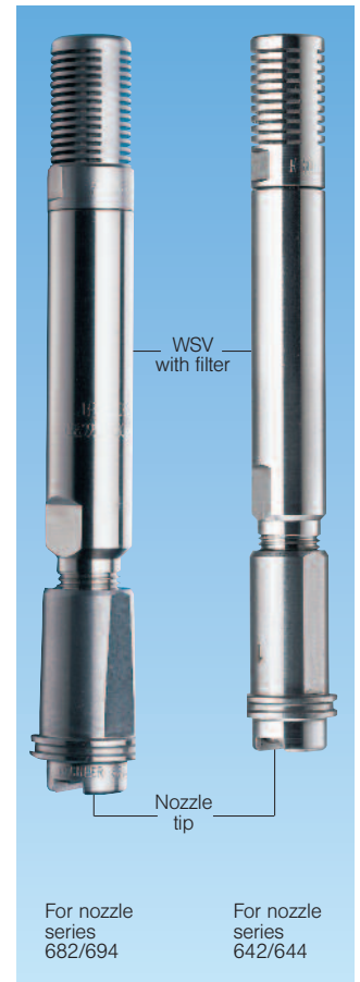
WSV Water Stop Valve, mounted with nozzle
